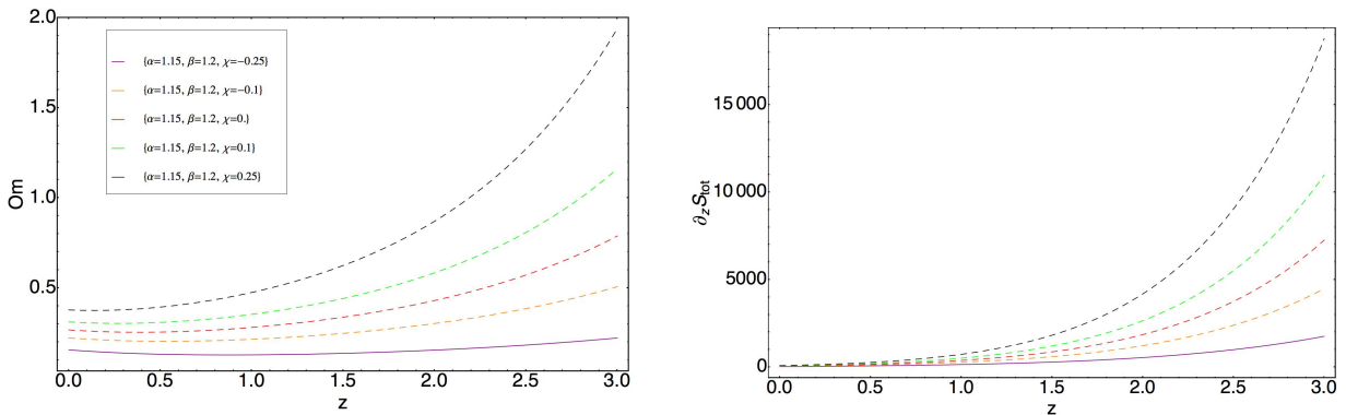
Figure 3: The graphical behavior of Om versus redshift z corresponds to the left plot. The right plot represents validity of generalized second law of thermodynamics. The case corresponds to non - interacting model
