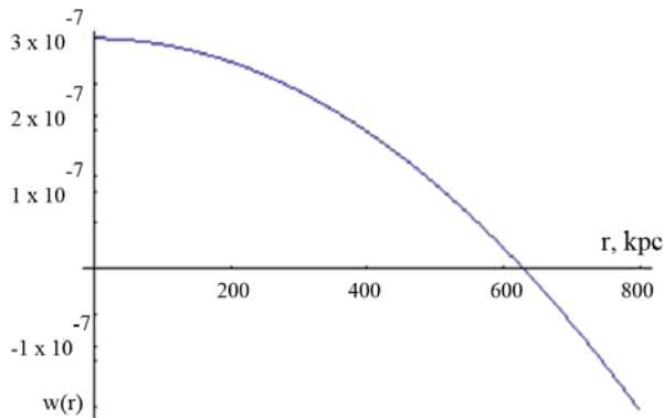
Fig. 4. The galactic halo radius
